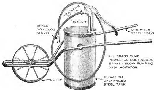
No. 50 Wheelbarrow Sprayer Double Action—Continuous Spray
